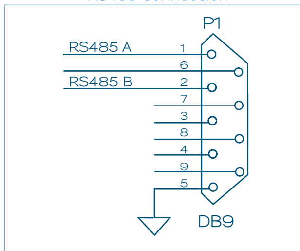
RS485 Connection
